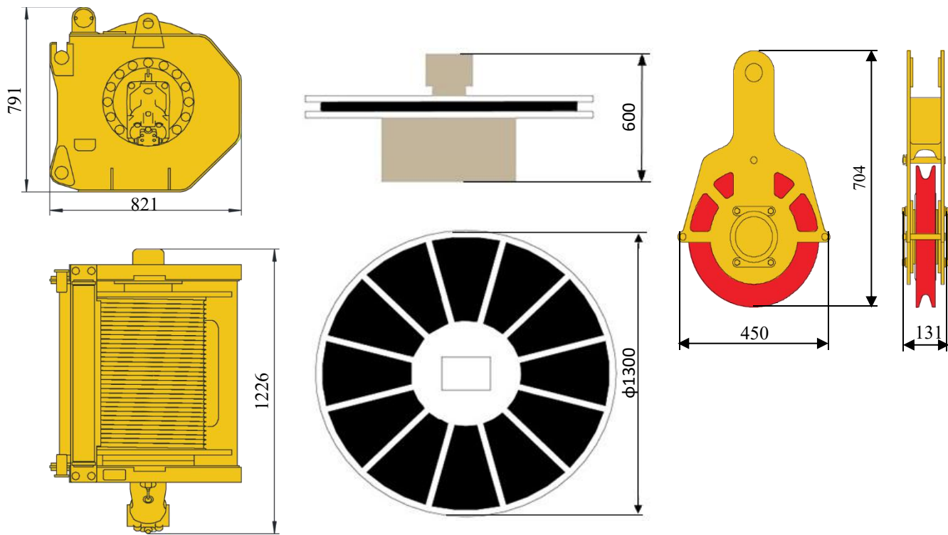
副起升机构 (含钢丝绳) 1409 kg Auxiliary winch (rope included) 1409 kg
