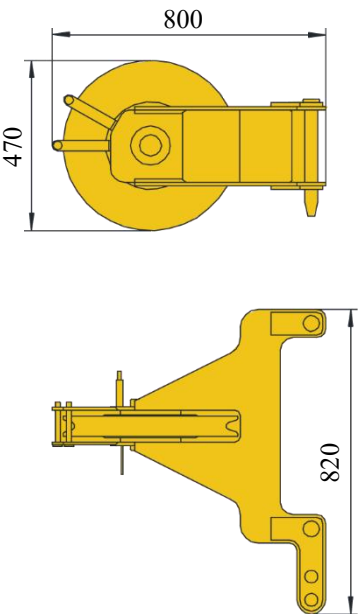
臂端单滑轮 60 kg Auxiliary sheave 60 kg
